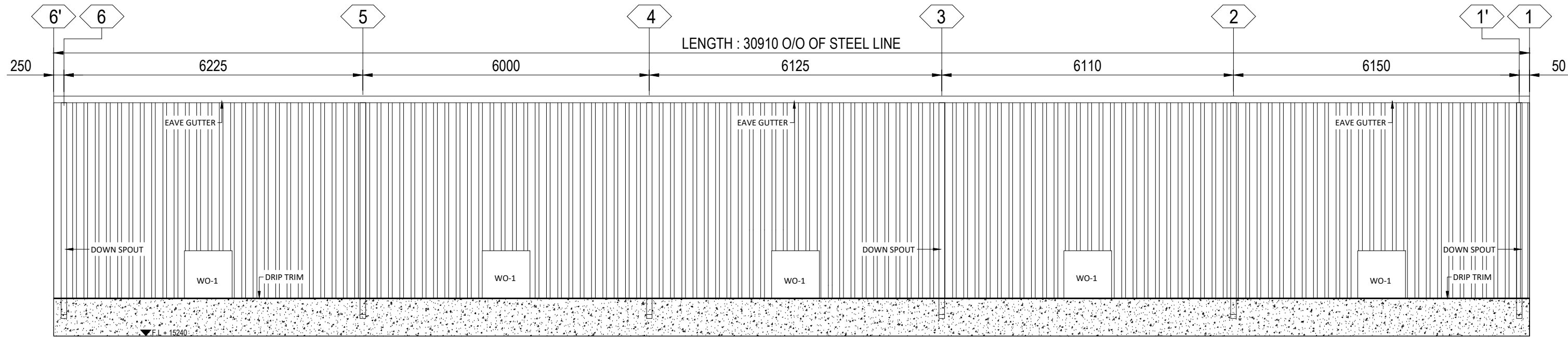
SIDE WALL SHEETING @ GRID - A
