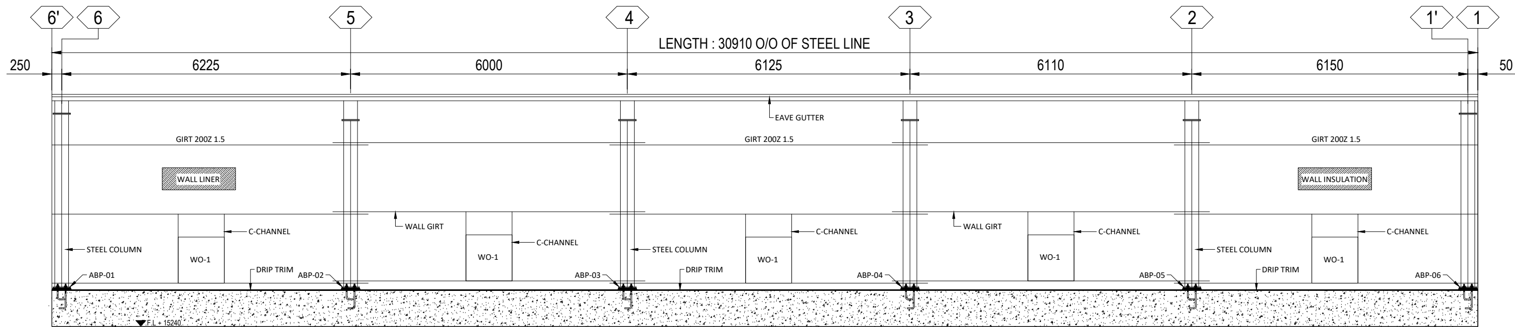
SIDE WALL FRAMING @ GRID - A
